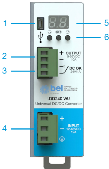
Figure 1. Front panel view
