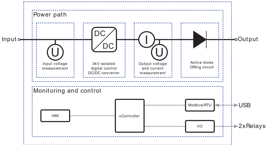
Figure 2. LDD240-WU simplified block diagram
