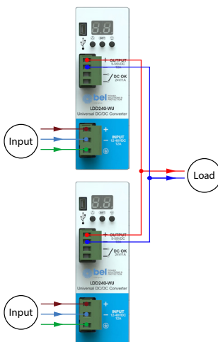
Figure 3. LDD240-WU parallel connection
