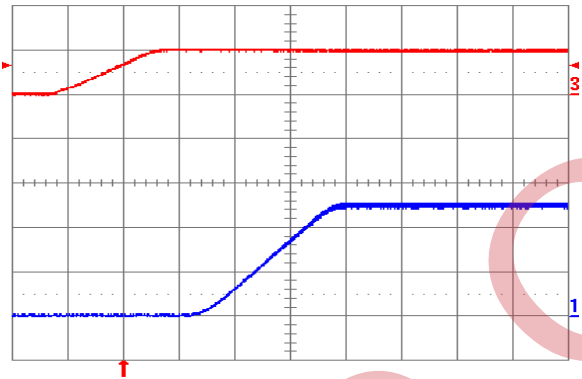
Fig. 2.5V.5: Turn-on transient for V_{out} = 2.5\text{ V} with application of V_{in} at full rated load current (resistive) and 47\text{ }\mu\text{F} external capacitance at V_{in} = 5\text{ V} . Top trace: V_{in} (5 V/div.); Bottom trace: output voltage (1V/div.); Time scale: 2 ms/div.
