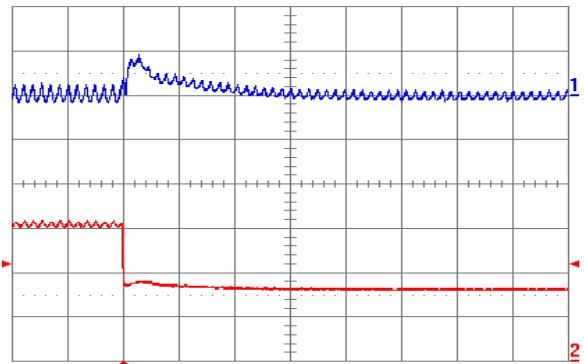
Fig. 0.7525V.8: Output voltage response for V_{out} = 0.7525 V to negative load current step change from 6 A to 3 A with slew rate of -5 A/ \mu s at V_{in} = 5 V. Top trace: output voltage (100 mV/div.); Bottom trace: load current (2 A/div.). C_o = 47 \mu F ceramic + 1 \mu F ceramic. Time scale: 20 \mu s/div.
