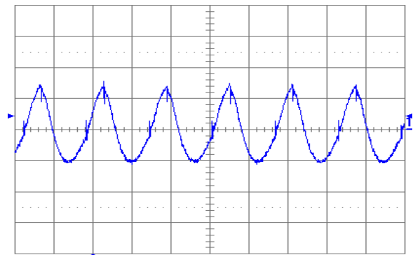
Fig. 1.2V.6: Output voltage ripple (20 mV/div.) at full rated load current into a resistive load with external capacitance 10\text{ }\mu\text{F} ceramic + 1\text{ }\mu\text{F} ceramic and V_{in} = 5\text{ V} for V_{out} = 1.2\text{ V} . Time scale: 2 \mu\text{s} /div.
