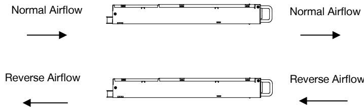
Figure 12. Airflow direction
