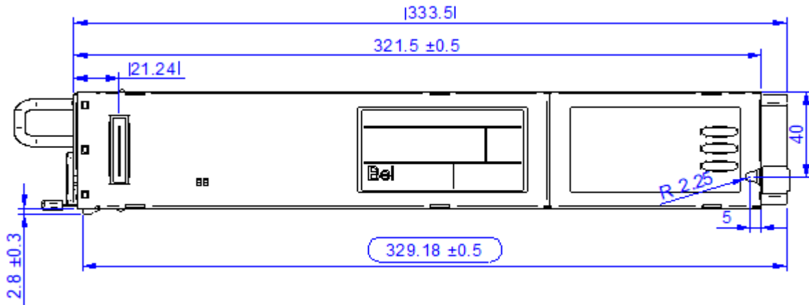
Figure 25. Top View
