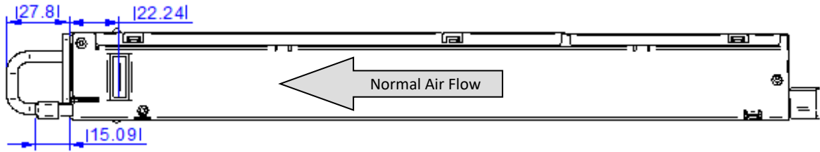
Figure 24. Side View 1
