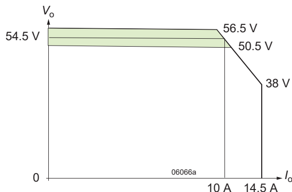
Fig. 12 Output characteristic of T1740 (typ.). The droop is shown in fig. 12.
