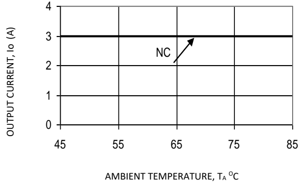
Figure 8. V_o = 1.2 V
