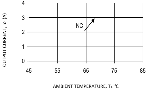
Figure 7. V_o = 0.6 V
