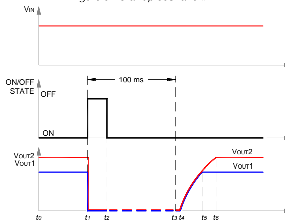
Figure 6. Startup scenario #3.
