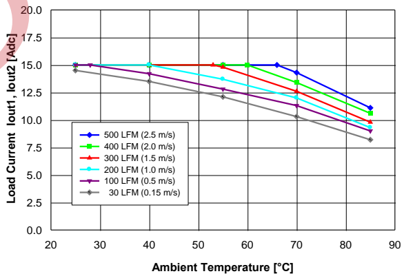
Figure 10. Available balanced load current ( I_{out1} = I_{out2} ) vs. ambient air temperature and airflow rates for converter mounted horizontally with V_{in} = 48 V, air flowing from pin 3 to pin 4 and maximum FET temperature \leq 120 °C.
