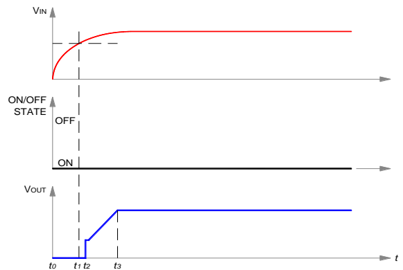
Figure 6. Start-up scenario #1.
