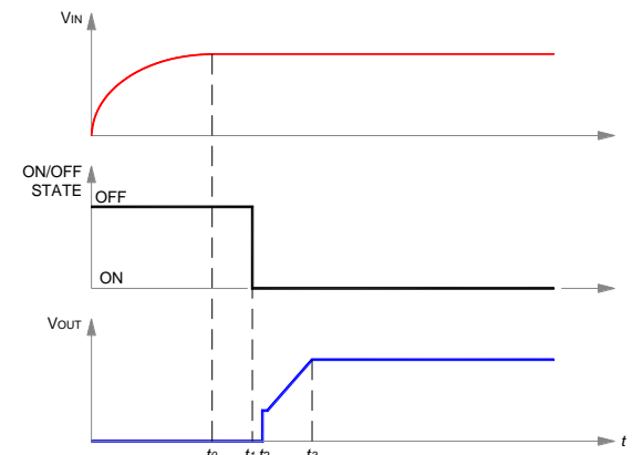
Figure 7. Startup scenario #2.
