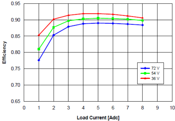
Figure 15. Efficiency vs. load current and input voltage for converter mounted horizontally with air flowing from pin 3 to pin 4 at a rate of 300 LFM (1.5 m/s) and T_a = 25\text{ }^\circ\text{C} .
