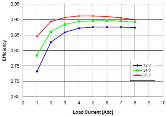
Figure 13. Efficiency vs. load current and input voltage for converter mounted vertically with air flowing from pin 3 to pin 1 at a rate of 300 LFM (1.5 m/s) and T_a = 25\text{ }^\circ\text{C} .
