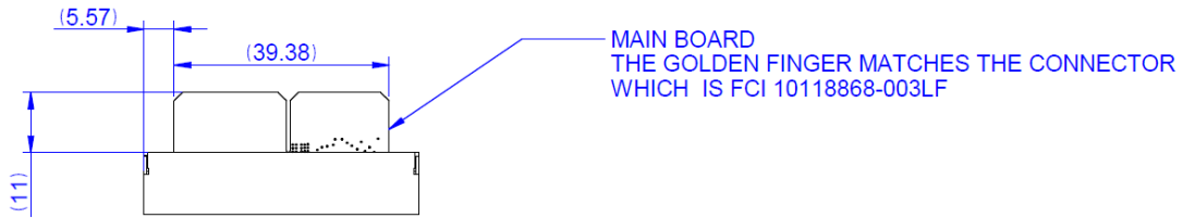
Figure 17. Mating Connector FCI 10118868-003LF
