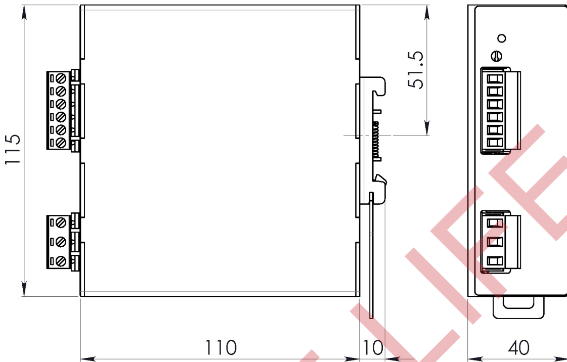
Figure 1. Mechanical Drawing
