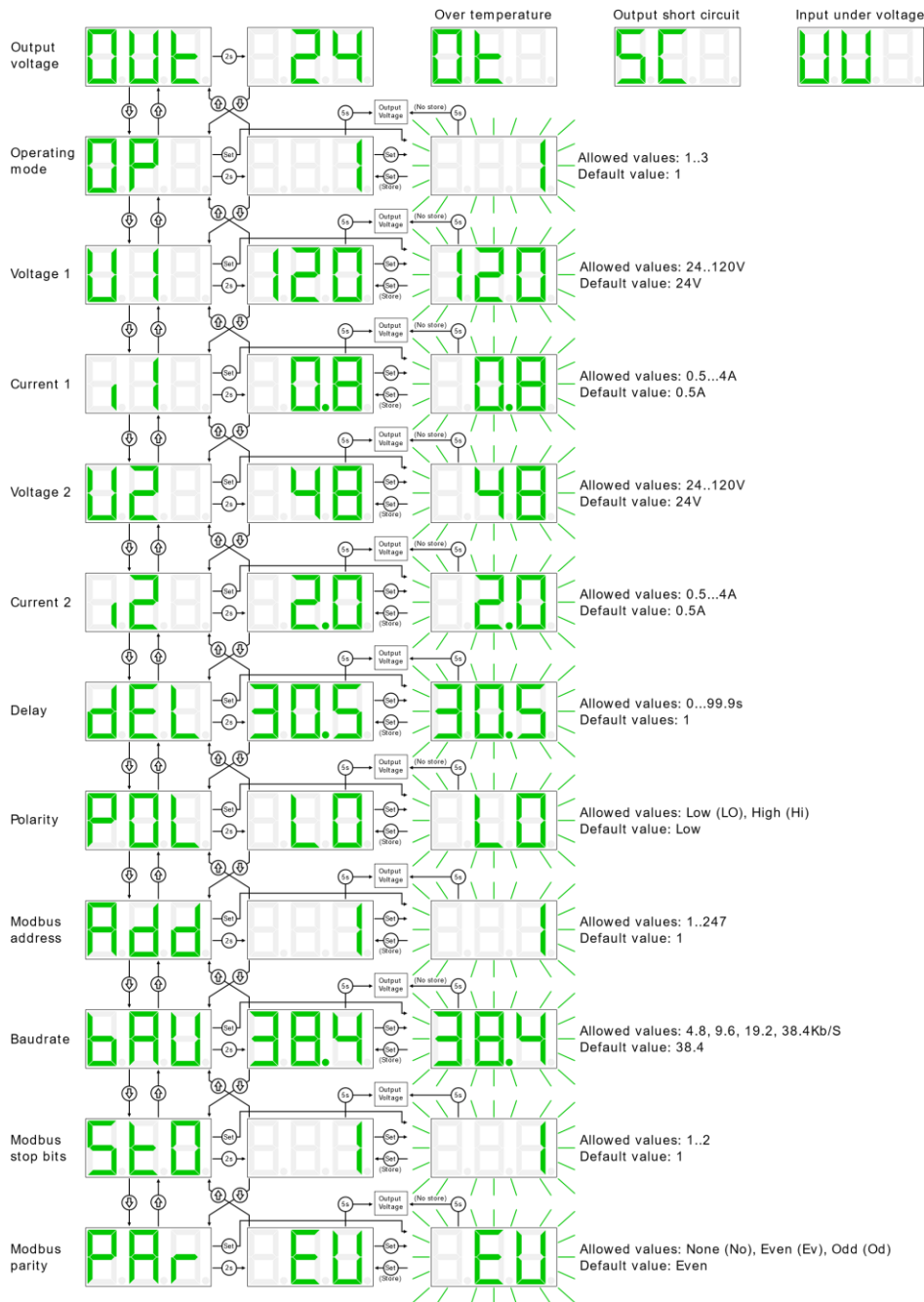
Figure 6: HMI
