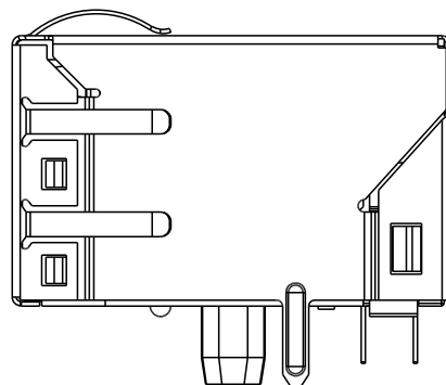
2250056-2 SHOWN (WITHOUT LED)
