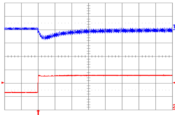
Fig. 0.7525V.7: Output voltage response for V_{out} = 0.7525\text{ V} to positive load current step change from 2.5 A to 5 A with slew rate of 5\text{ A}/\mu\text{s} at V_{in} = 12\text{ V} . Top trace: output voltage (100 mV/div.); Bottom trace: load current (2 A/div.). C_o = 100\text{ }\mu\text{F} ceramic. Time scale: 20\text{ }\mu\text{s/div.}
