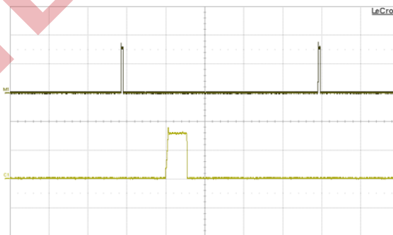
Fig. 17: Load current (top trace, 5 \text{ A}/\text{div} ., 100 \text{ ms}/\text{div} .) into a 10 \text{ m}\Omega short circuit during restart, at V_{in} = 48 \text{ V} . Bottom trace ( 5 \text{ A}/\text{div} ., 10 \text{ ms}/\text{div} .) is an expansion of the on-time portion of the top trace.
