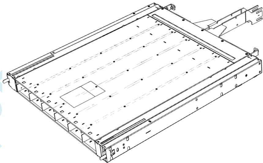
Figure 6. SPSTET4-07 Isometric View
