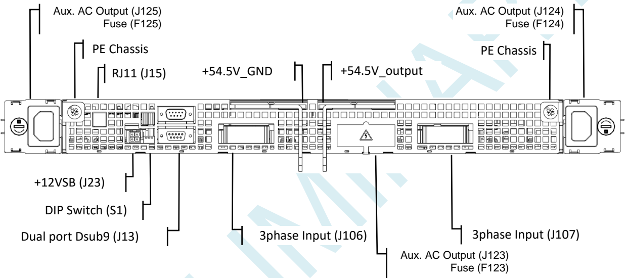
Figure 4. SPSTET4-07 Rear View
