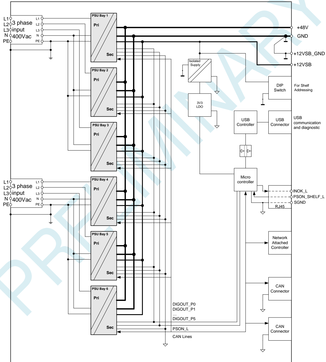
Figure 1. SPSTET4-07 Block Diagram (will be updated for Auxiliary AC Outlet)
