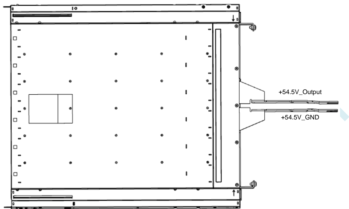
Figure 5. SPSTET4-07 Top View
