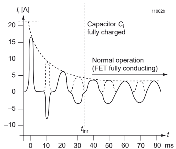
Fig. 33 Typ. inrush current with option E V_i = 230 VAC, f_i = 50 Hz, P_o = P_{o\text{ nom}}
