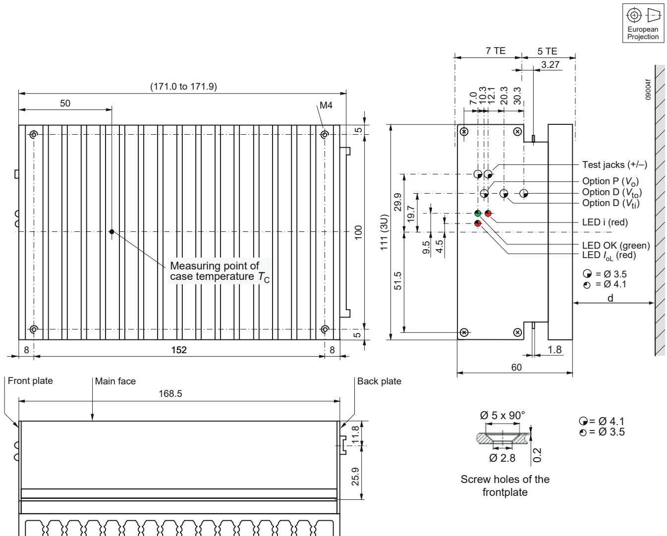
Fig. 27 Aluminum case S02 with heat sink; black finish (EP powder coated); weight approx. 1.25 kg
