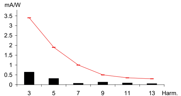
Fig. 8 Harmonic currents at the input: V_i=230 VAC, I_o = I_{o,nom} (LS4601).
