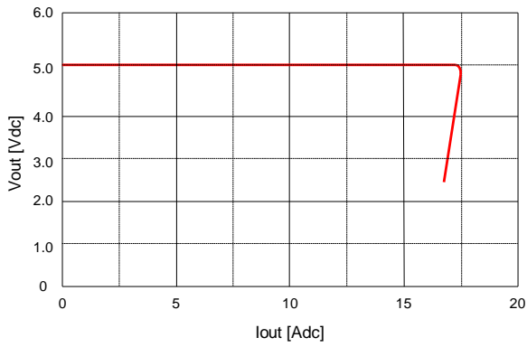
Figure 24. Output voltage vs. load current showing current limit point and converter shutdown point. Input voltage has almost no effect on current limit characteristic.
