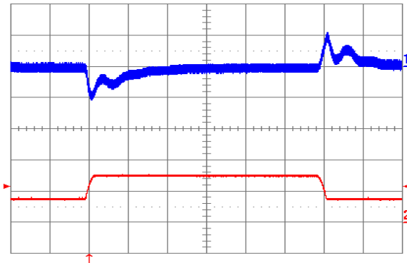
Figure 18. Output voltage response to load current step-change (3.75 A – 7.5 A – 3.75 A) at V_{in} = 24 V. Top trace: output voltage (100 mV/div). Bottom trace: load current (5 A/div.). Current slew rate: 0.1 A/ \mu s. C_o = 1 \mu F ceramic. Time scale: 0.2 ms/div.
