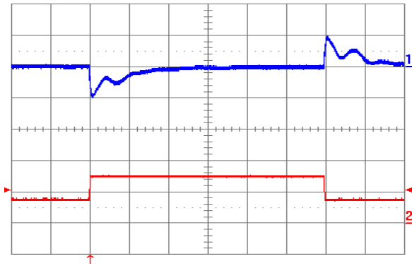
Figure 19. Output voltage response to load current step-change (3.75 A – 7.5 A – 3.75 A) at V_{in} = 24 V. Top trace: output voltage (100 mV/div.). Bottom trace: load current (5 A/div.). Current slew rate: 5 A/ \mu s. C_o = 450 \mu F tantalum + 1 \mu F ceramic. Time scale: 0.2 m
