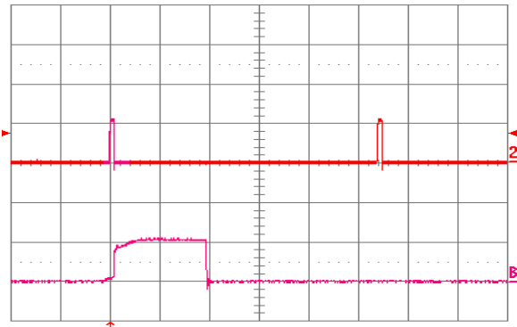
Figure 25. Load current (top trace, 20 A/div, 20 ms/div) into a 10 mΩ short circuit during restart, at Vin = 24 V. Bottom trace (20 A/div, 1 ms/div) is an expansion of the on-time portion of the top trace.
