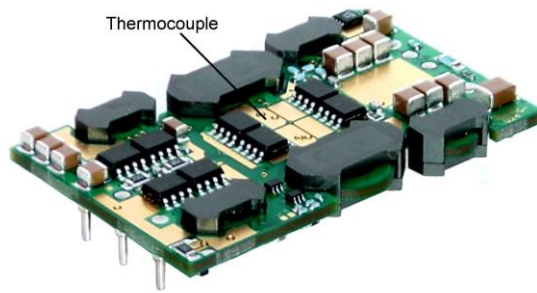
Figure 26. Location of the thermocouple for thermal testing.
