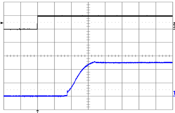
Figure 16. Turn-on transient at full rated load current (resistive) with no output capacitor at V_{in} = 24\text{ V} , triggered via ON/OFF pin. Top trace: ON/OFF signal (5 V/div.). Bottom trace: output voltage (2 V/div.). Time scale: 1 ms/div.
