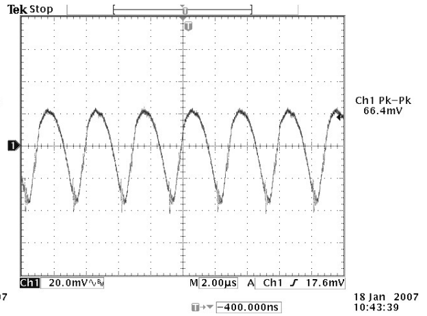
Figure 5. 48 Vdc input, 12 Vdc/5 A output
