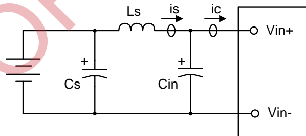
Figure 6. Test setup
