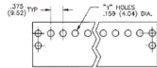
"Y" Terminal
