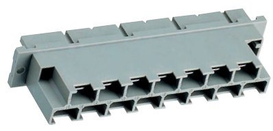
Fig. 21 H15 female connector with code key system
