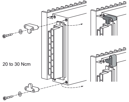
Fig. 23 Connector retention brackets HZZ01216-G
