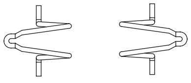
Fig. 22 Connector retention clips HZZ01209-G
