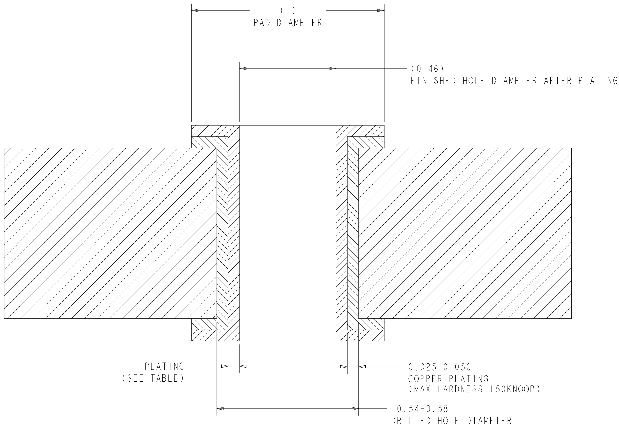
RECOMMENDED HOLE DIMENSIONS FOR SIGNAL CONTACTS
