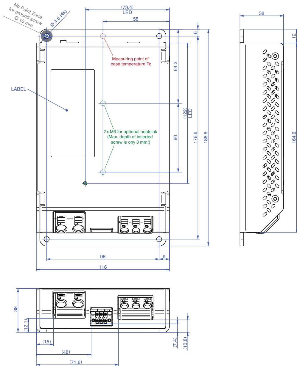
Fig. 8 Case for XRCM300, Standard version, Aluminum, EP black anodized; 800 g.
