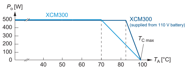
Fig. 4 Typical output power derating versus temperature; horizontal mounting position, free convection cooling.
