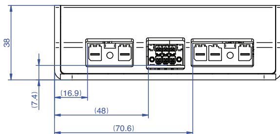
Fig. 9 Mechanical dimensions XRCM300 (Version with option K)
