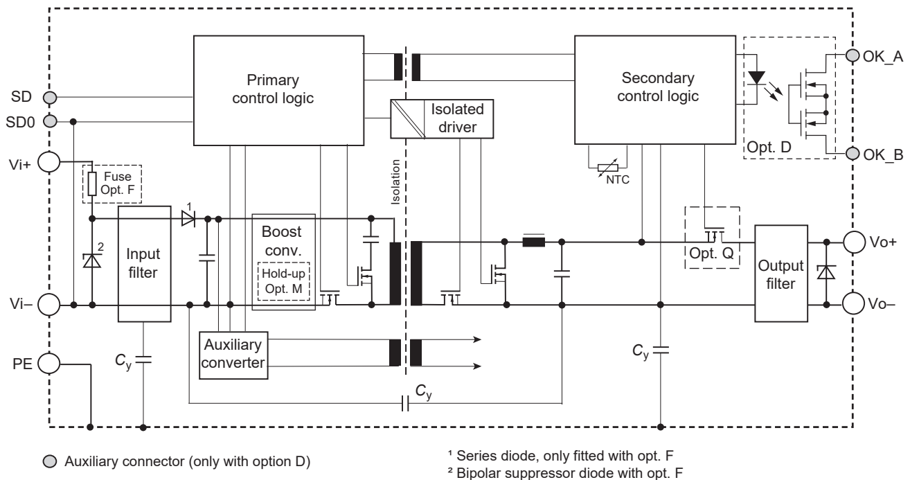
Fig. 1 Block diagram
