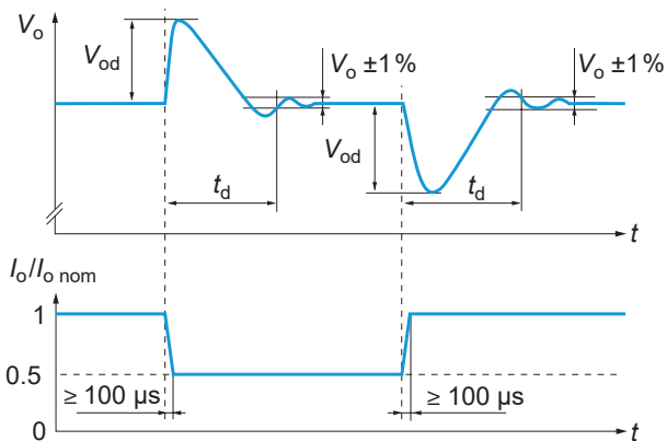
Fig. 2 Typical dynamic load regulation of output voltage
