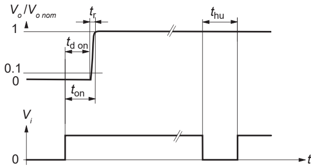
Fig. 7 Typical output response to V_i
