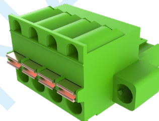
Fig. 12b Female connector for option K, 4 poles (HZZ00151-G)
