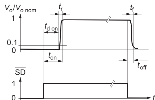
Fig. 6 Typical output response to the SD-signal
