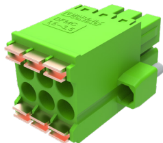
Fig. 11 Female connector 6 pins (Phoenix Contact 1790302)
