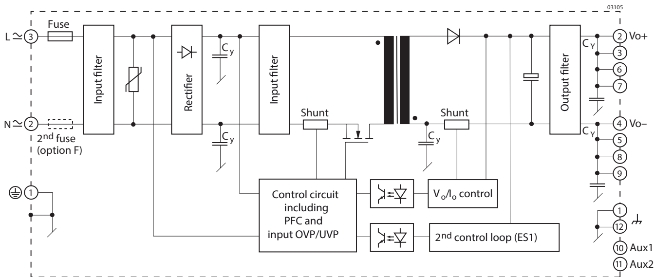
Fig. 1 LXR 375 W single-output converter.
