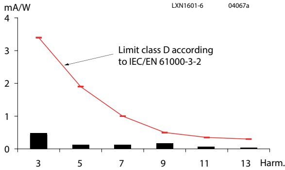
Fig. 4 Harmonic currents at input current, measured at V_i = 230 \text{ VAC} , I_o = I_{o \text{ nom}} (LXN1601-6)
