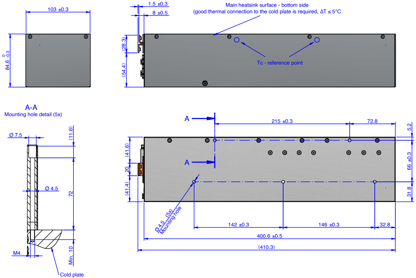
Figure 3. Mechanical Drawing
