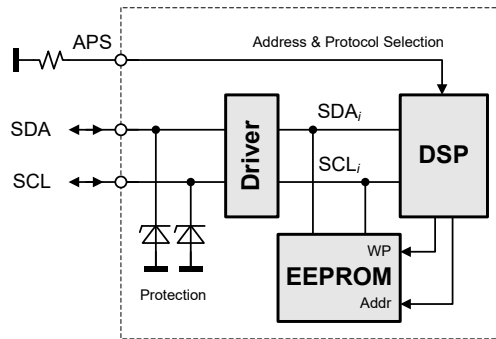
Figure 19. I2C Bus to DPS and EEPROM
