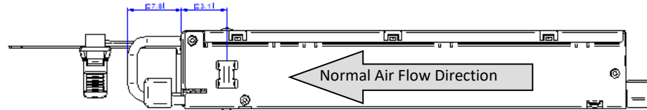
Figure 25. Side View
