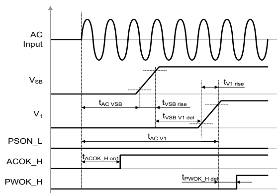
Figure 11. AC turn-on timing
