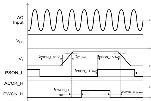
Figure 14. PSN_L and PWOK_H turn-on/off timing
