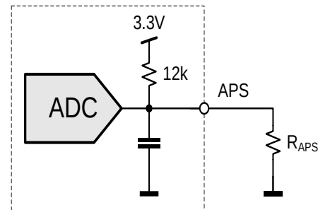
Figure 34. I 2 C address and protocol setting
