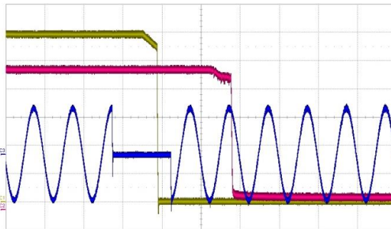
Figure 12. AC drop out 30 ms (20 ms/div) CH1: V_1 (2 V/div) CH2: V_{SB} (1 V/div) CH3: V_{in} (200 V/div)
