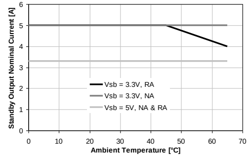
Figure 22. Temperature derating on V_{SB}
