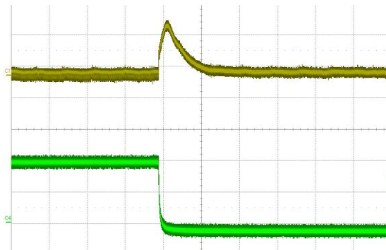
Figure 15. Load transient V_1 , 30 to 5 A (500 \mu s/div) CH1: V_1 (200 mV/div), CH4: I_1 (10 A/div)
