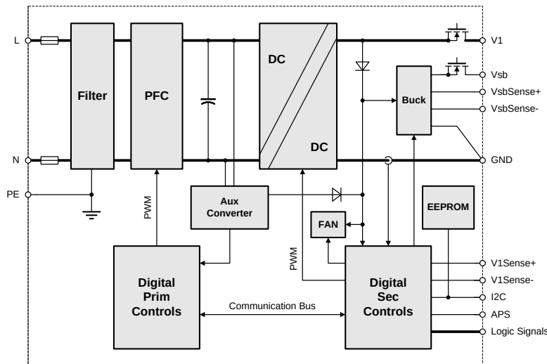
Figure 1. PFE600-12-054xA Block Diagram
