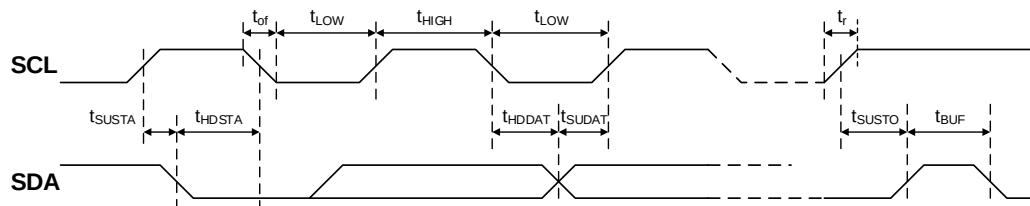
Figure 33. I 2 C / SMBus Timing
