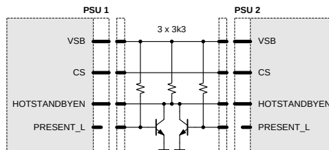
Figure 31. Recommended hot-standby configuration
