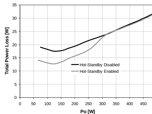
Figure 30. PSU power losses with/without hot-standby mode
