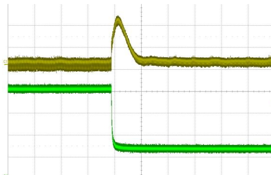
Figure 17. Load transient V_1 , 45 to 20 A (500 \mu s/div) CH1: V_1 (200 mV/div), CH4: I_1 (10 A/div)
