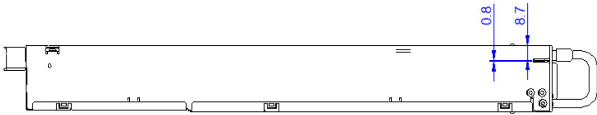
Figure 43. Side View 2
