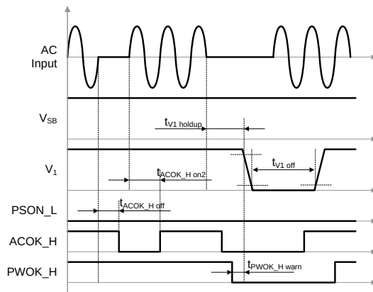
Figure 26. AC short dips
