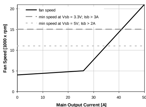
Figure 38. Fan speed vs. main output load
