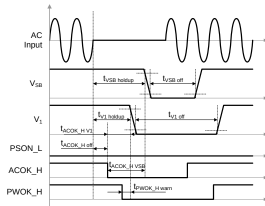
Figure 27. AC long dips
