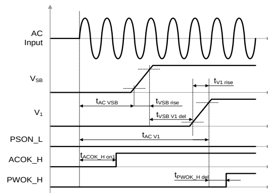
Figure 25. AC turn-on timing
