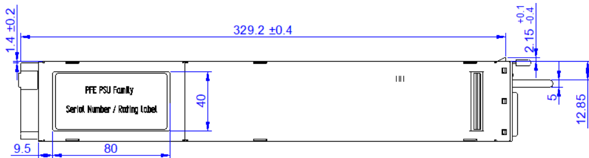
Figure 42. Top View
