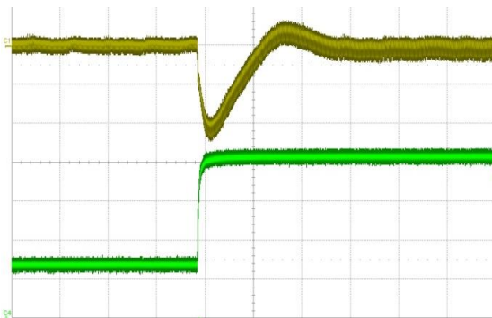
Figure 16. Load transient V_1 , 20 to 45 A (500 \mu s/div) CH1: V_1 (200 mV/div), CH4: I_1 (10 A/div)
