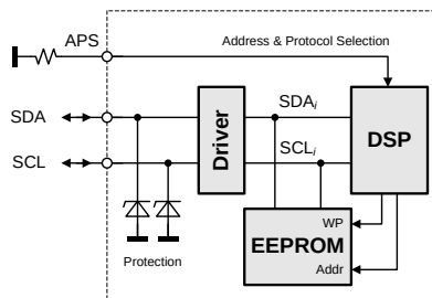
Figure 35. I 2 C Bus to DSP and EEPROM
