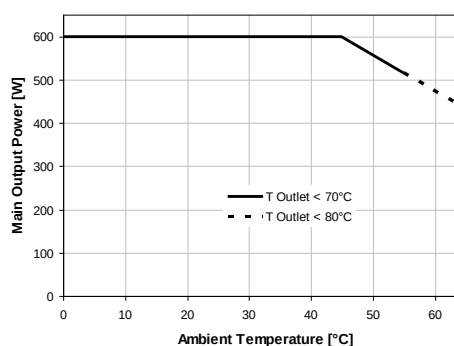
Figure 39. Thermal derating for PFE600-12-054NA
