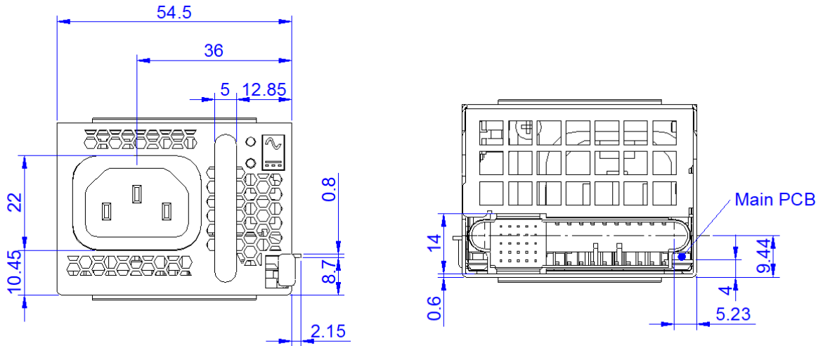
Figure 44. Front and Rear View
