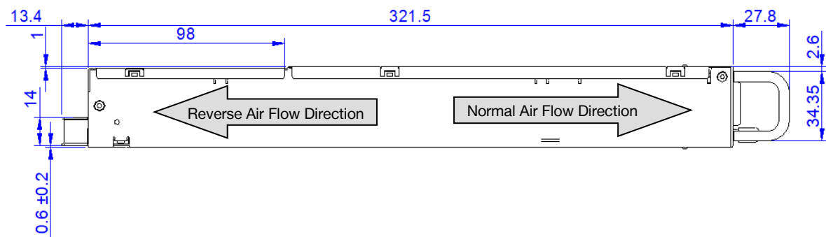
Figure 41. Side View 1
