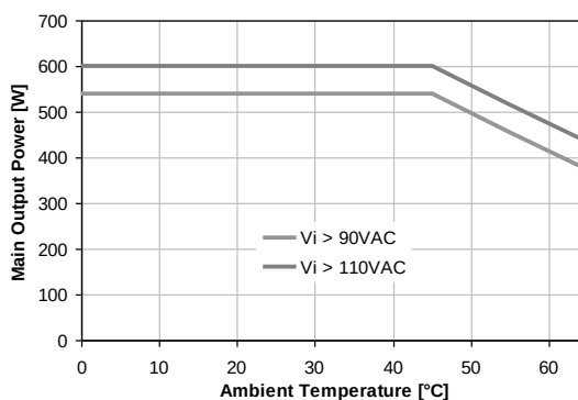
Figure 40. Thermal derating for PFE600-12-054RA
