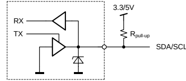
Figure 32. Physical layer of communication interface
