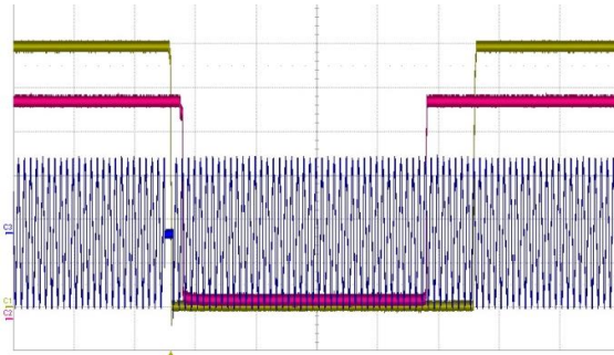
Figure 13. AC drop out 30ms (200 ms/div), V_1 restart after 1s CH1: V_1 (2 V/div) CH2: V_{SB} (1 V/div) CH3: I_1 (200 V/div)
