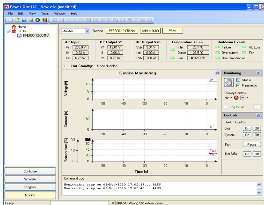
Figure 36. Monitoring dialog of the I2C Utility
