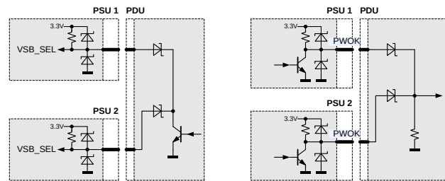
Figure 23. Interconnection of Signal Pins
