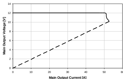
Figure 18. Current Limitation on V_1 ( V_1 = 230 VAC)
