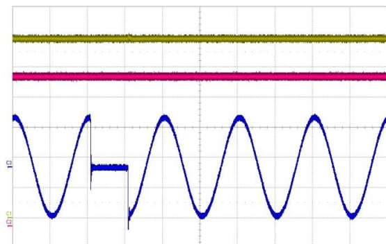
Figure 11. CH1: V_1 (2 V/div) CH2: V_{SB} (1 V/div) CH3: V_{in} (200 V/div)
