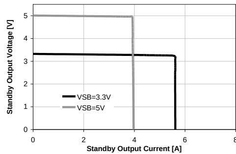
Figure 21. Current limitation on V_{SB}
