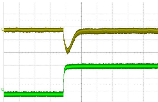
Figure 14. Load transient V_1 , 5 to 30 A (500 \mu s/div) CH1: V_1 (200 mV/div), CH4: I_1 (10 A/div)
