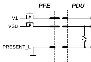
Figure 24. PRESENT_L signal pin
