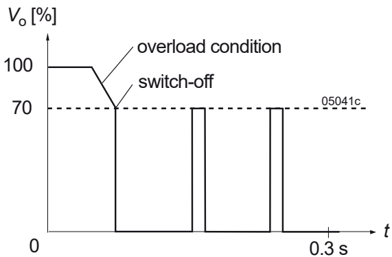
Fig. 8 Overload switch-off (hiccup mode); typical values
