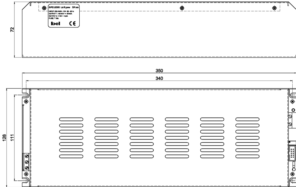
Figure 2 - Mechanical Drawing
