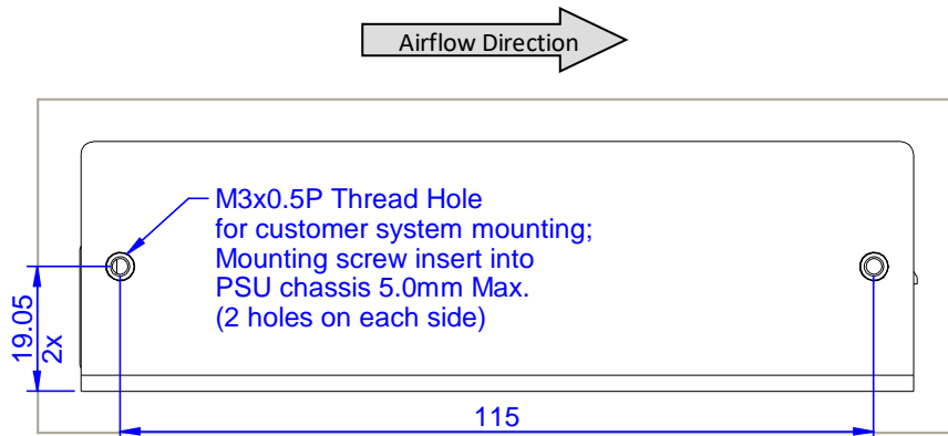
Figure 17: Side view 1
