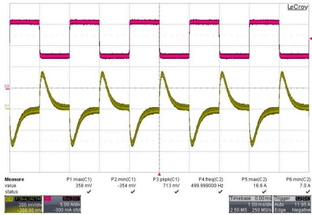
Figure 14: Load transient V_o (1.0ms/div), 8.5A <-> 17A, 2Aμs CH1: V_o (200 mV/div) CH2: I_o (5 A/div)
