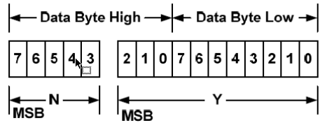
Figure 13. Linear Data Format Data Bytes
