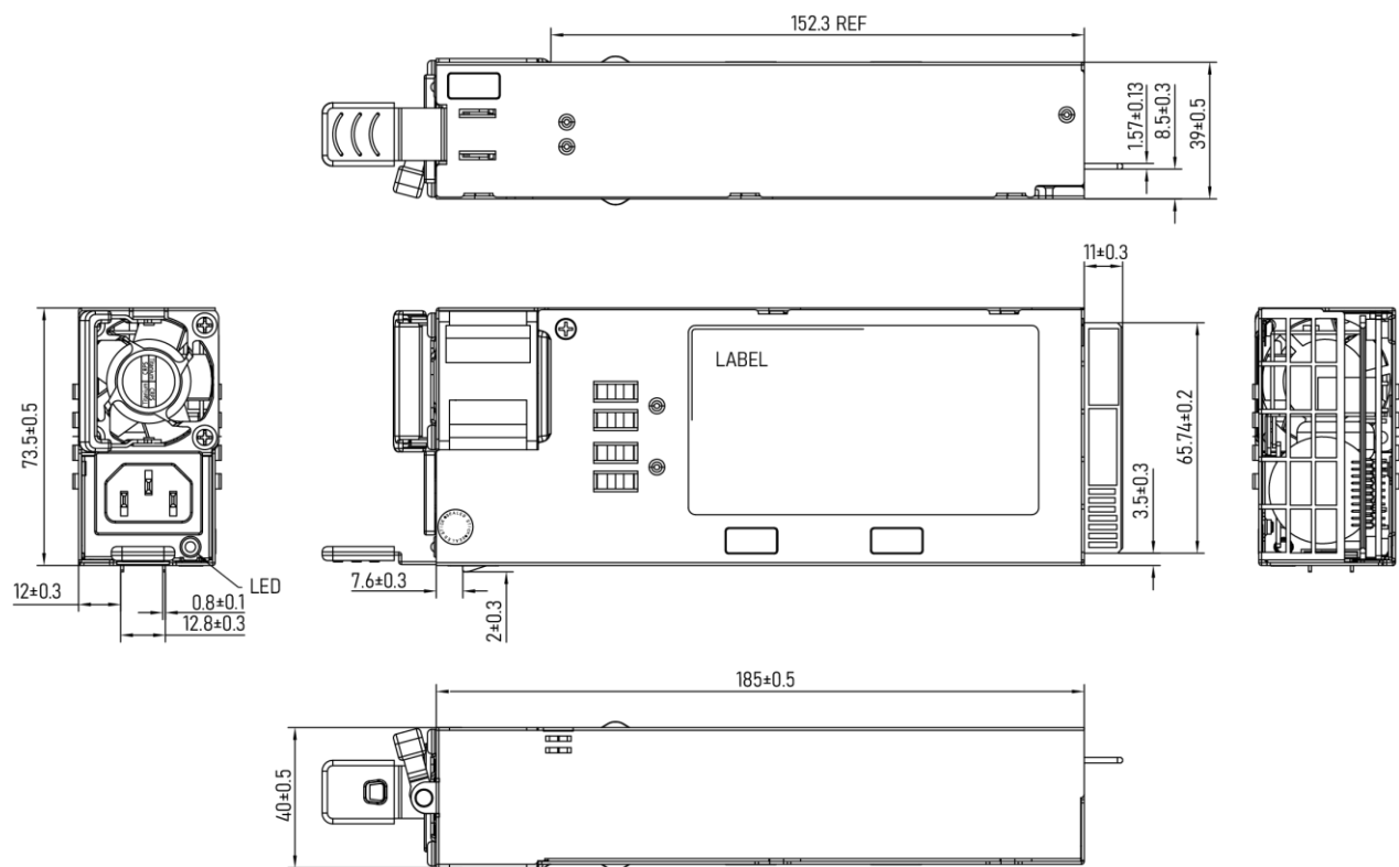
Figure 19. Mechanical Drawing
