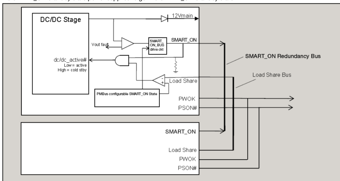
SMART_ON BUS LOAD SHARE DC/DC_ACTIVE# SMART_ON STANDBY POWER SUPPLY STATE(S) High < V_{SMART\_ON} High SMART_ON Standby Low < V_{SMART\_ON} Low Active High > V_{SMART\_ON} Low Active Low > V_{SMART\_ON} Low Active
