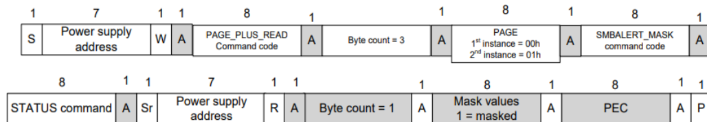
Figure 8. PAGE_PLUS_READ command.
