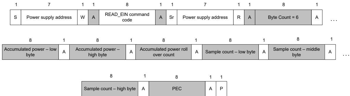
Figure 11. READ_EIN Command
