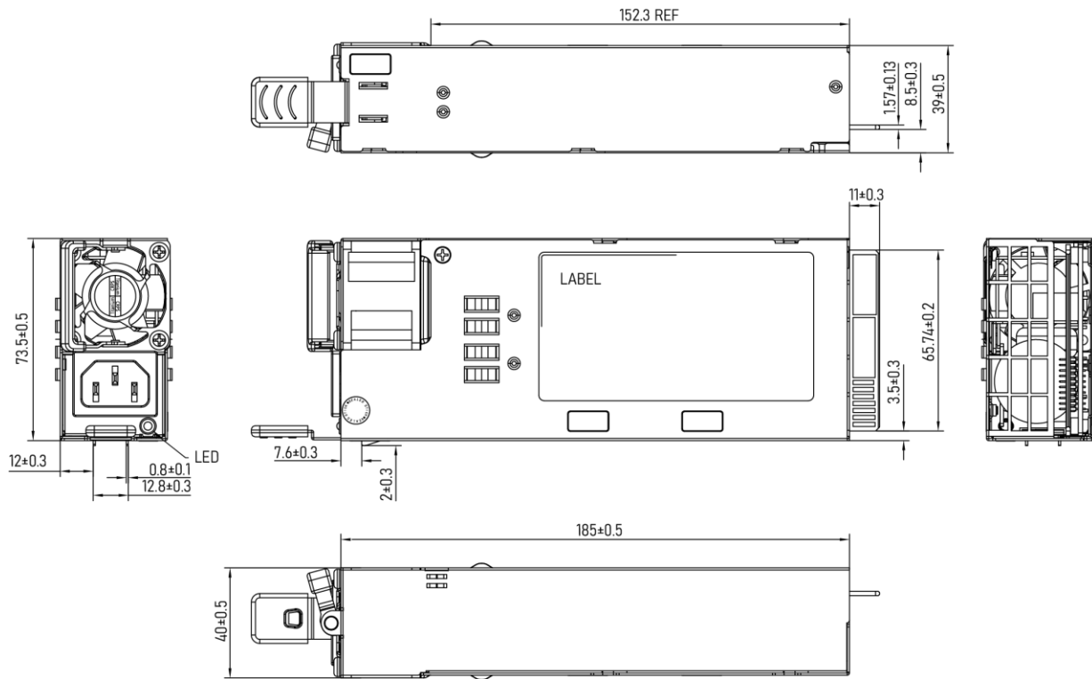
Figure 19. Mechanical Drawing
