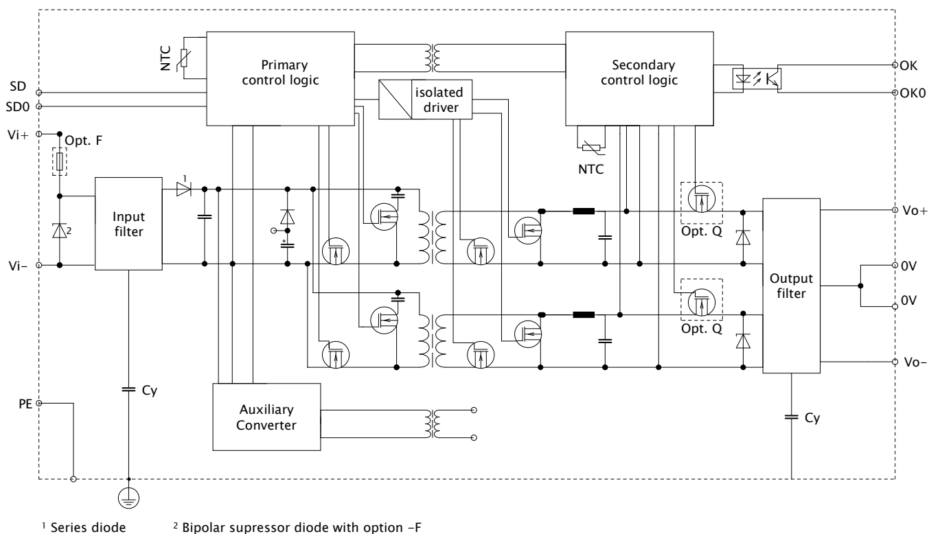
Fig. 1 Block diagram
