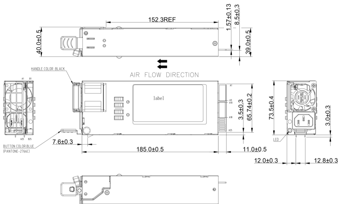
Figure 5. Mechanical Drawing
