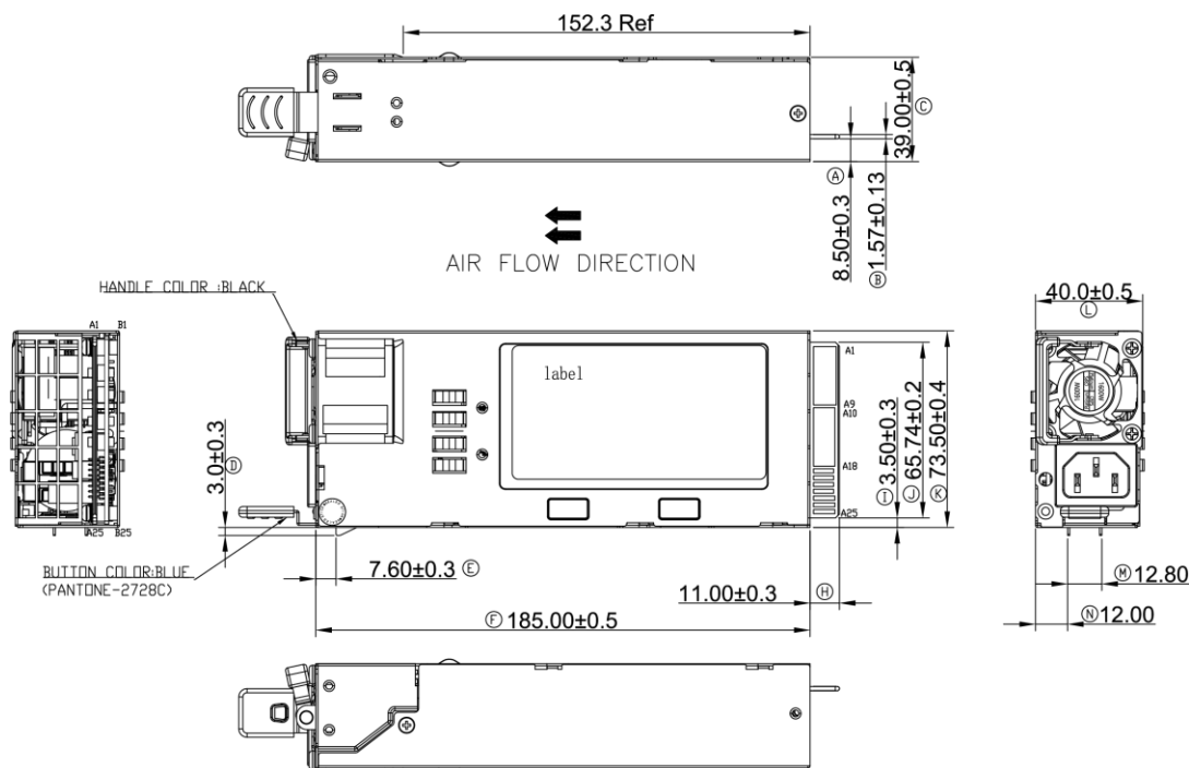
Figure 5. Mechanical Drawing
