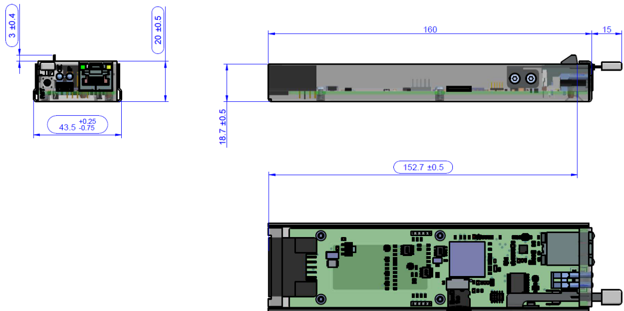
Figure 5. Front, side, top view
