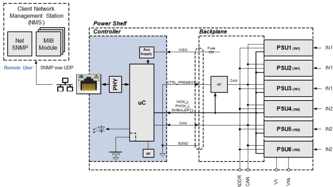
Figure 1. NAC3006-02 block diagram and its integration into SPSTET4 and SPSTET4V3 power shelves
