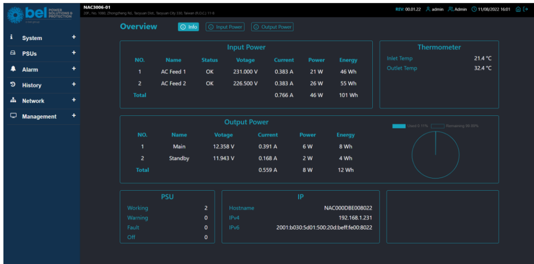
Figure 3. NAC3006-02 Web interface
