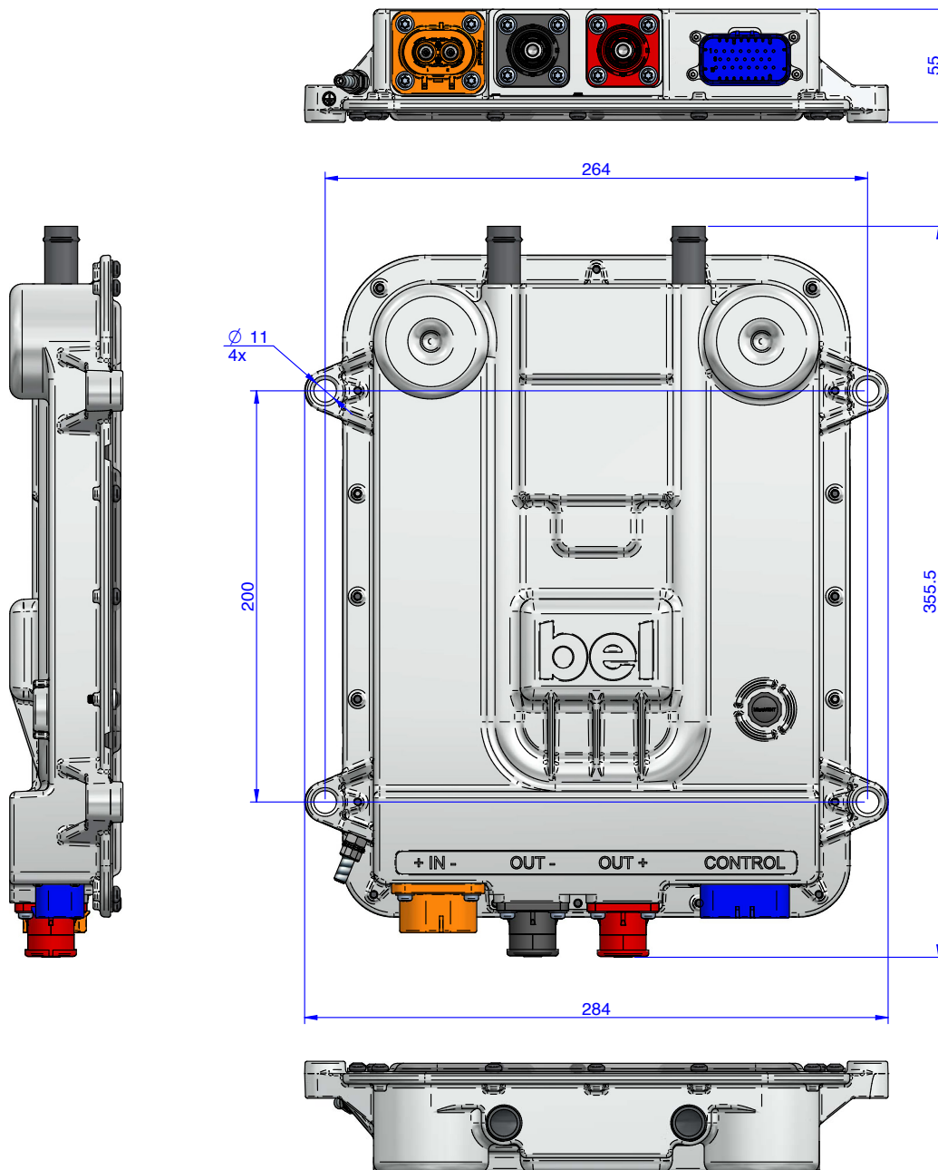
Figure 7. Mechanical Drawing
