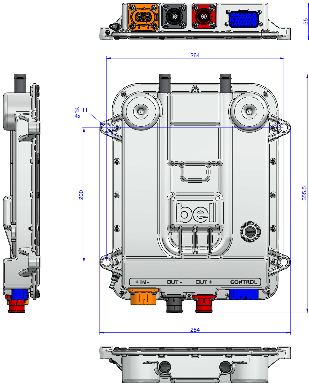
Figure 7. Mechanical Drawing
