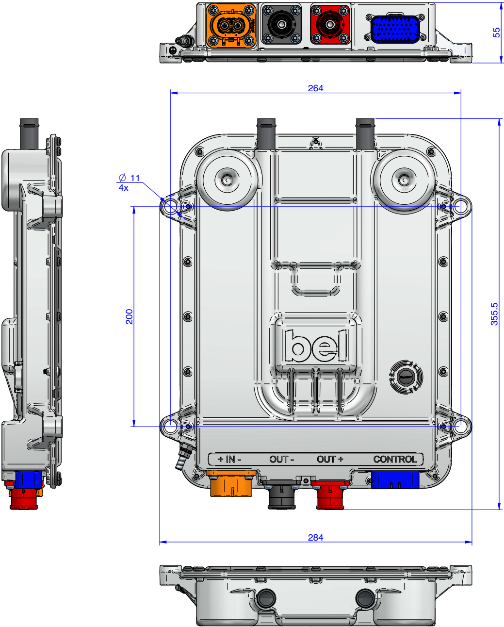
Figure 7. Mechanical Drawing
