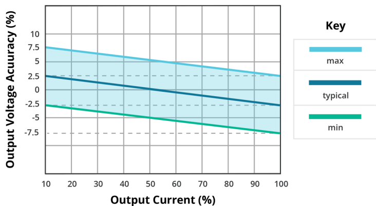
OUTPUT REGULATION CURVE VQA3S-S15-D15-S (+Vo)
