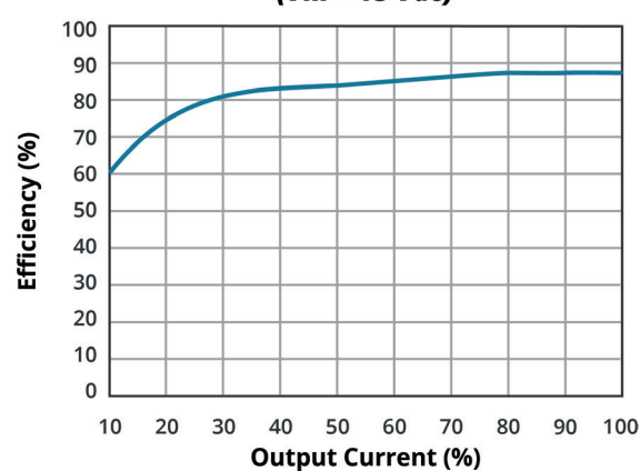
EFFICIENCY VS OUTPUT LOAD ( V_{in} = 15\text{ Vdc} )
