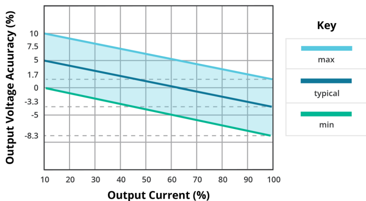
OUTPUT REGULATION CURVE VQA3S-S15-D20-S (+Vo)
