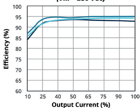
EFFICIENCY VS OUTPUT LOAD ( V_{in} = 230 \text{ Vac} )
