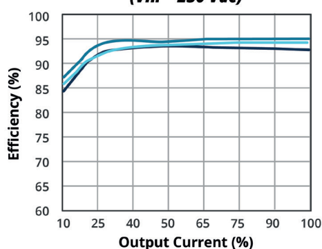
EFFICIENCY VS OUTPUT LOAD ( V_{in} = 230 \text{ Vac} )
