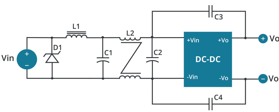
Figure 2 Recommended Circuit for EN55022 Class B
