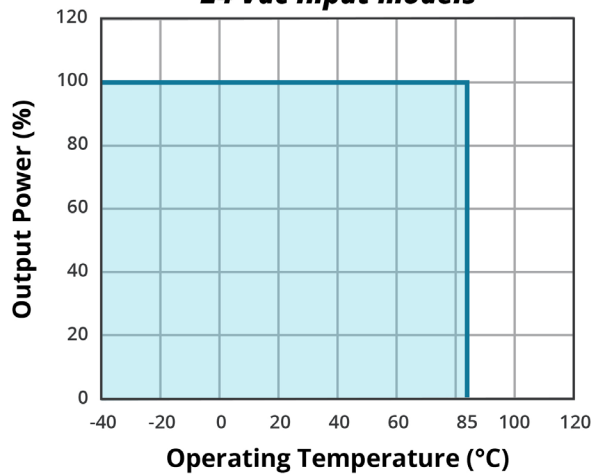
TEMPERATURE DERATING CURVE 24 Vdc Input models
