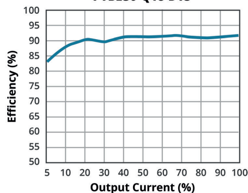
EFFICIENCY VS OUTPUT LOAD ( V_{in} = 48V ) PYBE30-Q48-D15
