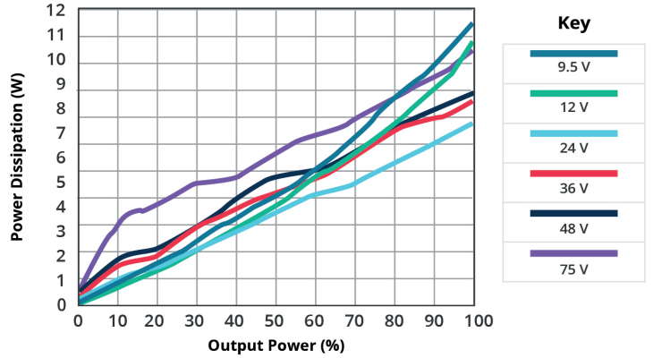
POWER DISSIPATION VS OUTPUT POWER PST75W-36-S28B (at 25°C)
