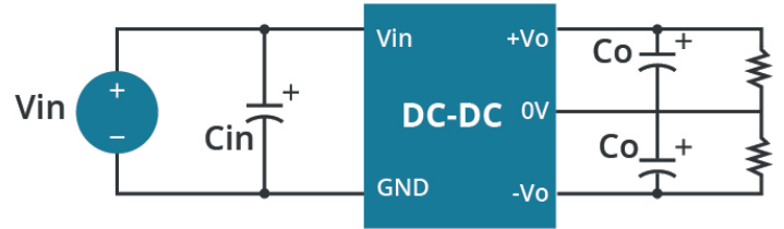
Figure 2 Dual output
