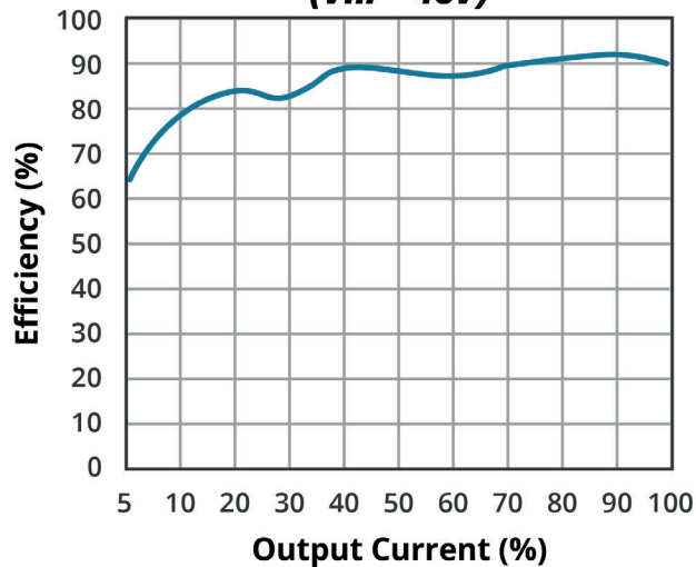
EFFICIENCY VS OUTPUT LOAD PDQE15-Q48-D24-U (Vin = 48V)
