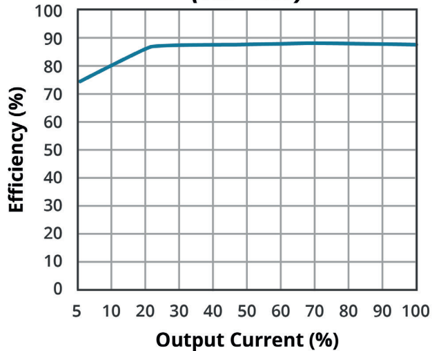
EFFICIENCY VS OUTPUT LOAD PDQE15-Q24-D5-U (Vin = 24V)
