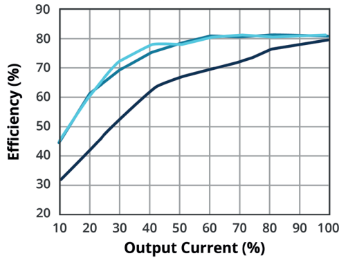
EFFICIENCY VS OUTPUT LOAD PDQ2-D5-S15-S
