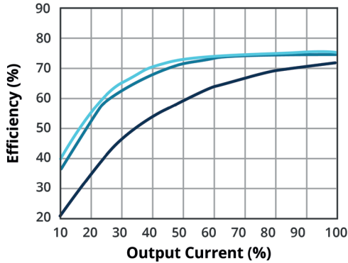
EFFICIENCY VS OUTPUT LOAD PDQ2-D5-S3-S
