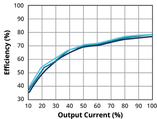
EFFICIENCY VS OUTPUT LOAD PCN1-S12-D5-S
