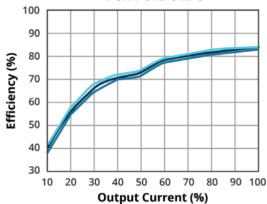
EFFICIENCY VS OUTPUT LOAD PCN1-S12-S12-S
