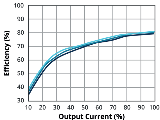
EFFICIENCY VS OUTPUT LOAD PCN1-S5-D15-S
