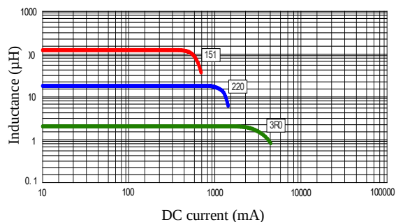
SCRH6D28 Inductance decrease by current
